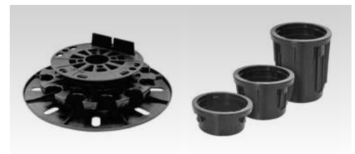
Height adjustable pedestals - 35 mm to 60 mm. Extension inserts - 25 mm, 50 mm and 100 mm.
