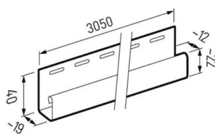
"J" TRIM (U CAPPING)
