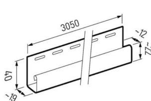
"J" TRIM (U CAPPING)
